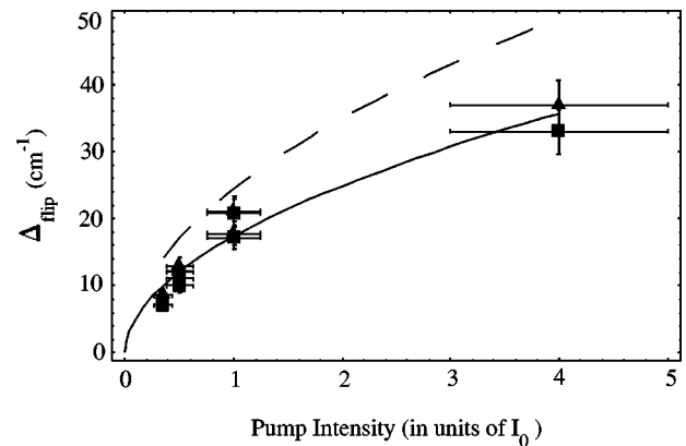
FIG. 10. \Delta_{flip} vs pump-laser intensity I ; I_0 corresponds to \sim 20 \text{ cm}^{-1} ; P_{Ar} = 1 \text{ Torr} ; triangles correspond to detunings \omega_L > \omega_o ; squares correspond to detunings \omega_L < \omega_o ; solid line is fit to data; dashed line is fit to prediction based on calculated cross sections for collisional transfer. The solid line and the dashed line show the same power-law dependence.
